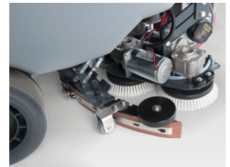
Four small disk brushes, with a vacuum rail directly behind them allow for a short design and a very tight turning circle
