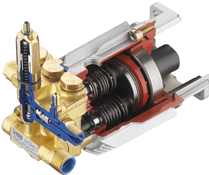
Wobble-plate pump
