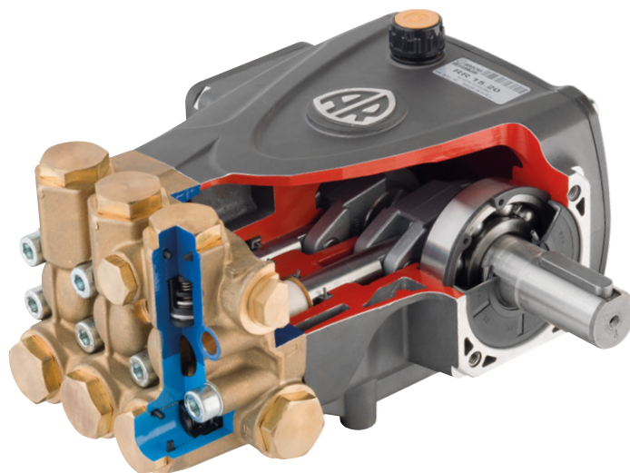
Crank pump
